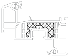
Thermomodul
